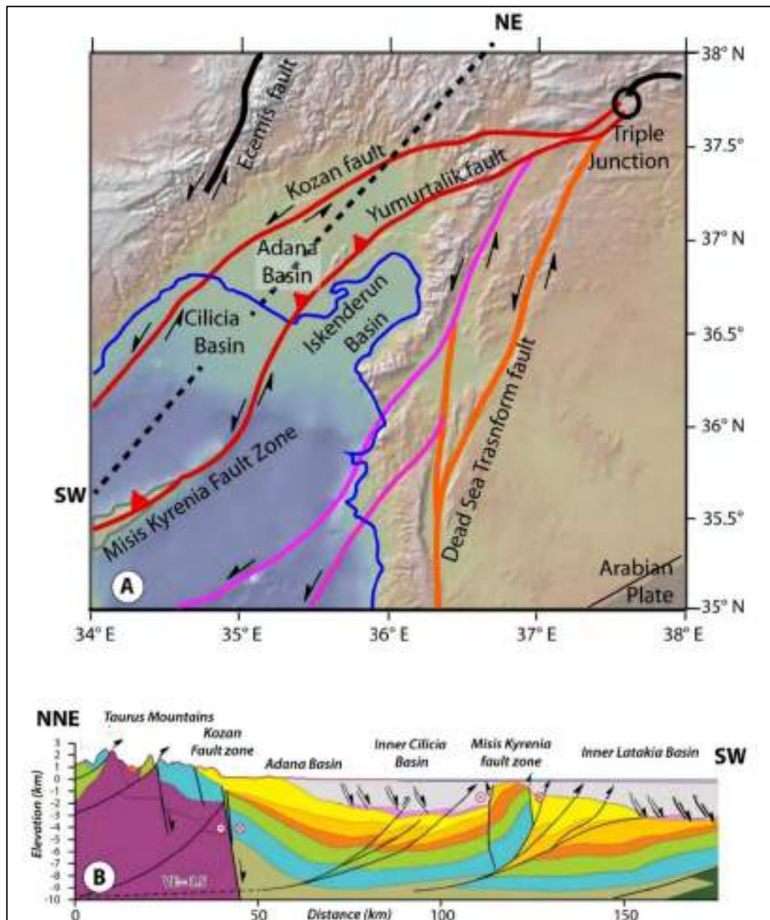
Figure 2. Structural constraints of the evolution of the Çukurova delta, from Göksu river mouth to İskenderun basin. A. Main fault lineaments (background map source: GeomapApp software), B. Geological cross-section from Kozan highlands toward Cyprus Sea. Source: modified from Aksu et al. (2021).
