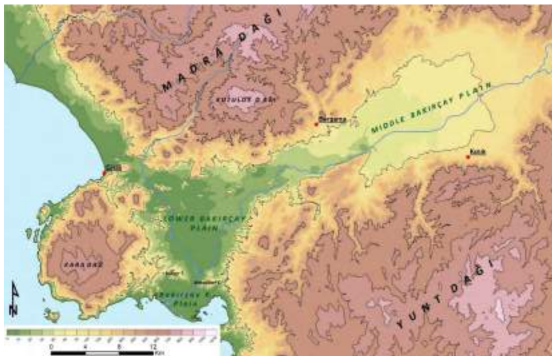
Figure 2. Location of Middle and Lower Bakırçay plains and its delta.
