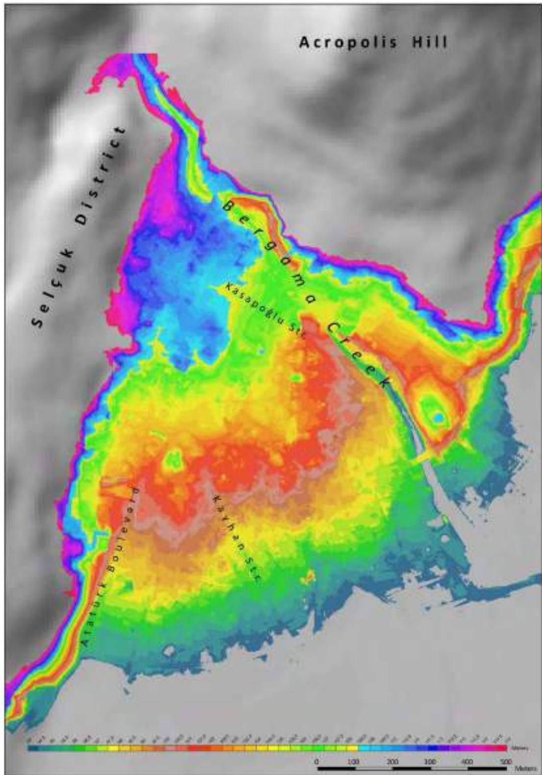
Figure 7. Proximal part of Bergama alluvial fan.
