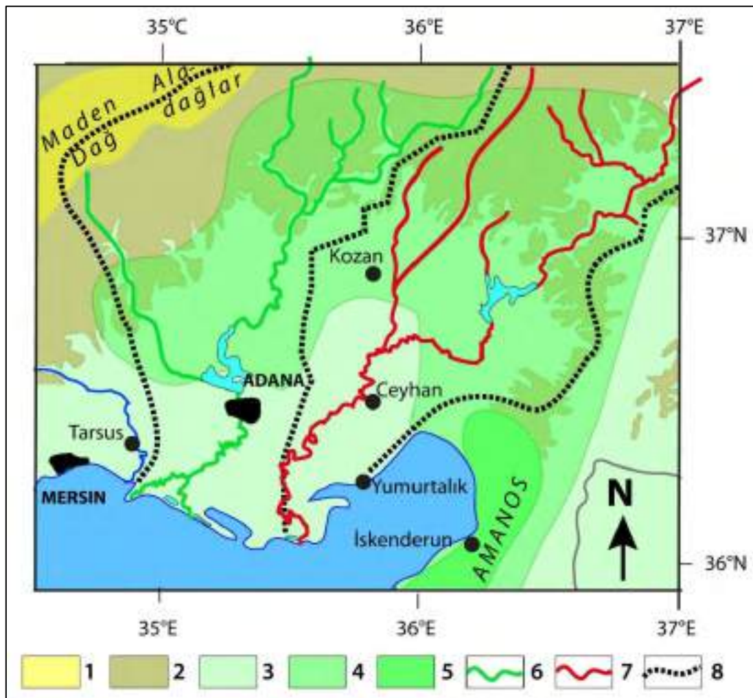
Figure 5. Mean annual precipitations over areas drained by rivers toward the Adana and the Cilician plain. Legend: 1. Area with P < 300 mm/yr; 2. Area with 300 < P < 600 mm/yr; 3. Area with 600 < P < 800 mm/yr; 4. Area with 800 < P < 1000 mm/yr; 5. Area with P > 1000 mm/yr. Source: modified from Atalay et al. (2014) and Sensoy (2016).
