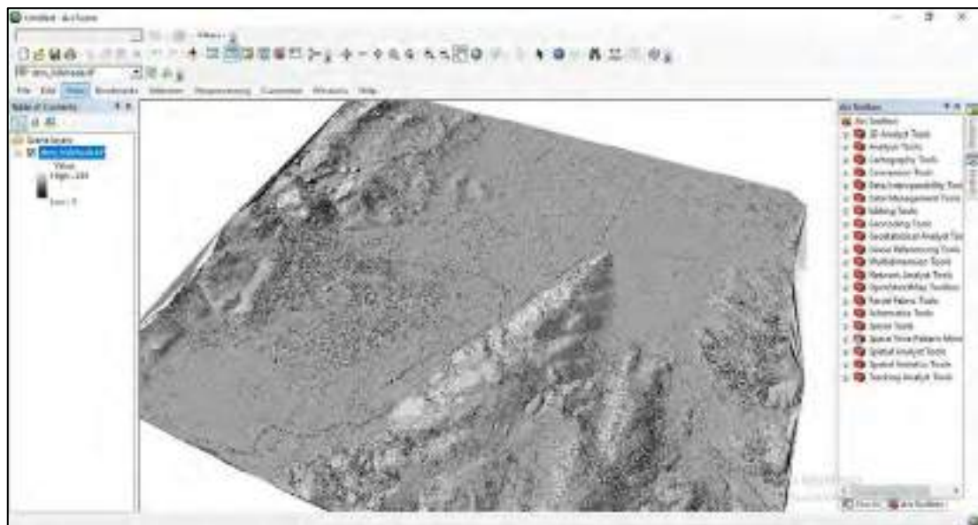
Figure 1. Hillshade map of Bergama plain its environs created from LiDAR data.
