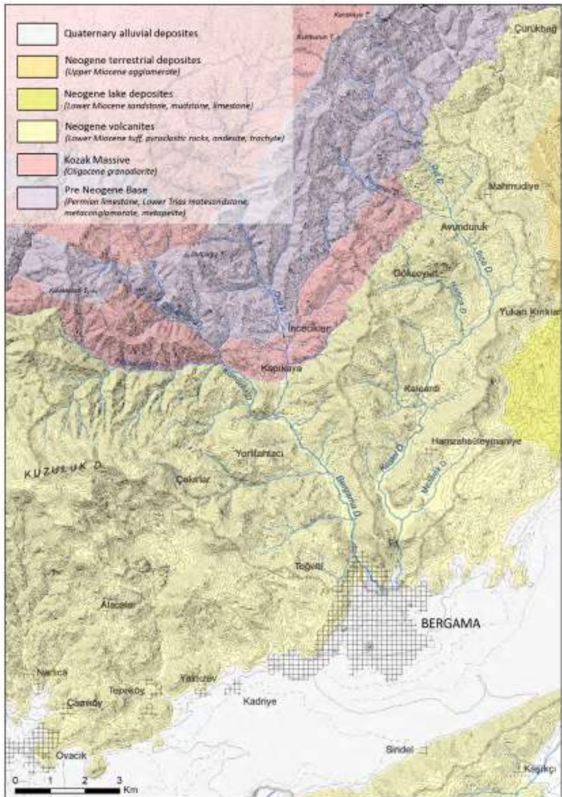
Figure 6. Geological map of the Bergama and Kestel drainage basins.
